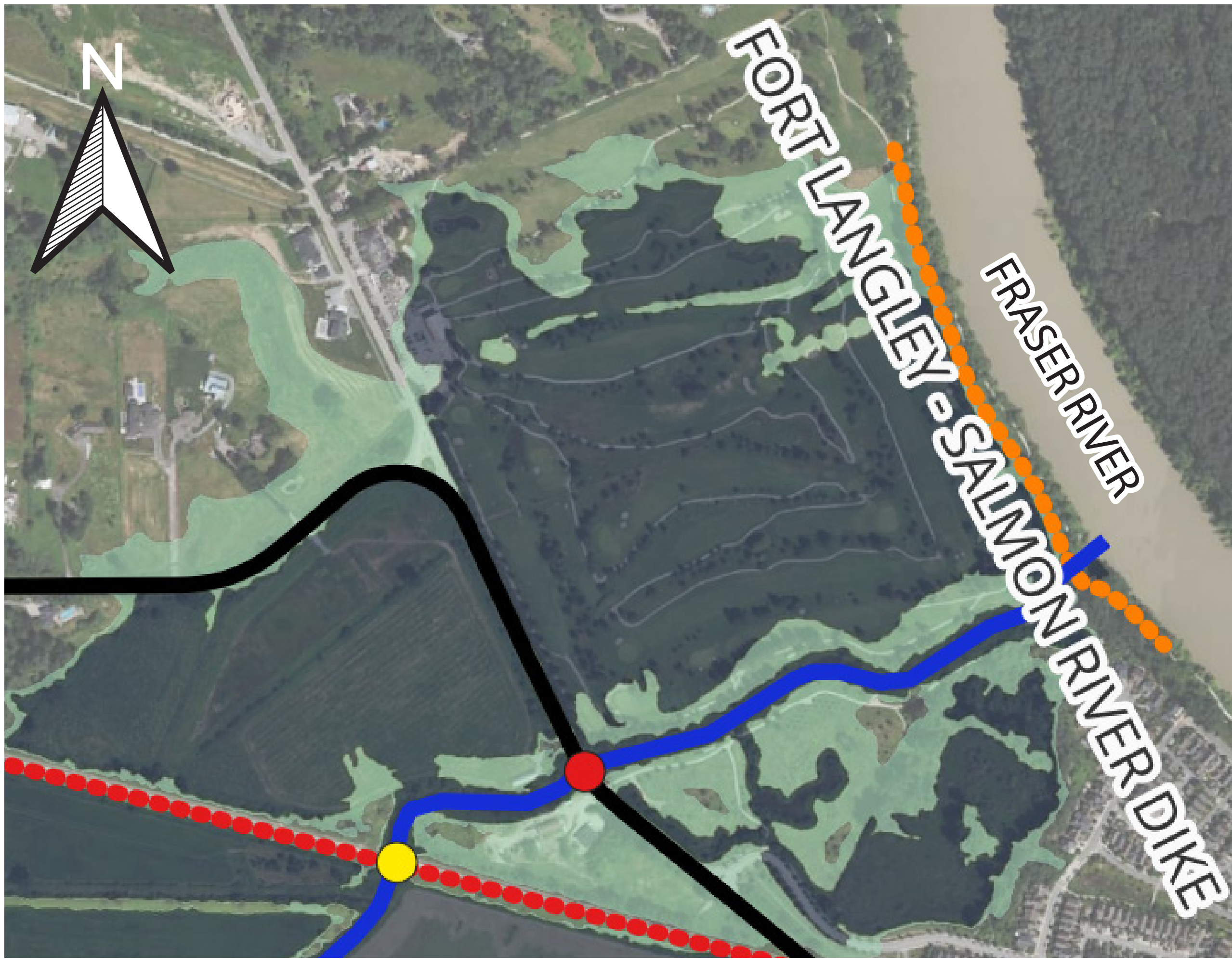
Proposed Drainage Upgrade — Winter Design Scenario
